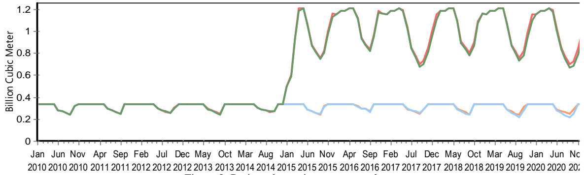
Figure 2: Projected reseivour storage volume
